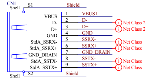
USB3.0 Type A Female
